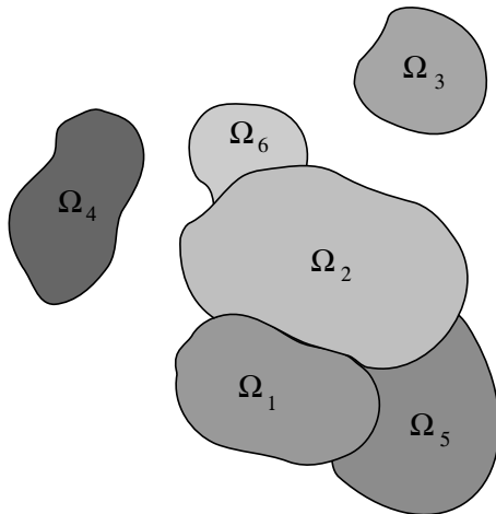
FIGURE 2. Multi-region configuration in \mathbb{R}^2 .
